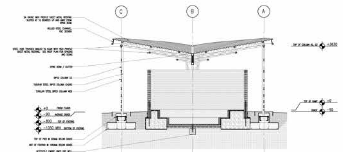
2 SMALL CLASSROOM CROSS-SECTION SCALE: 1:50
